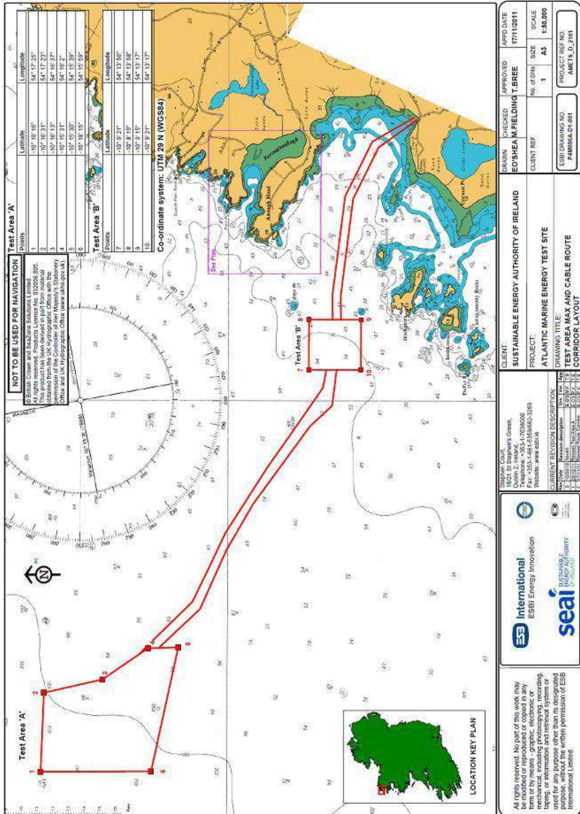
Figure 1-1: Proposed wave energy test site layout
