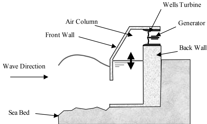
Fig 1: Outline of an OWC
