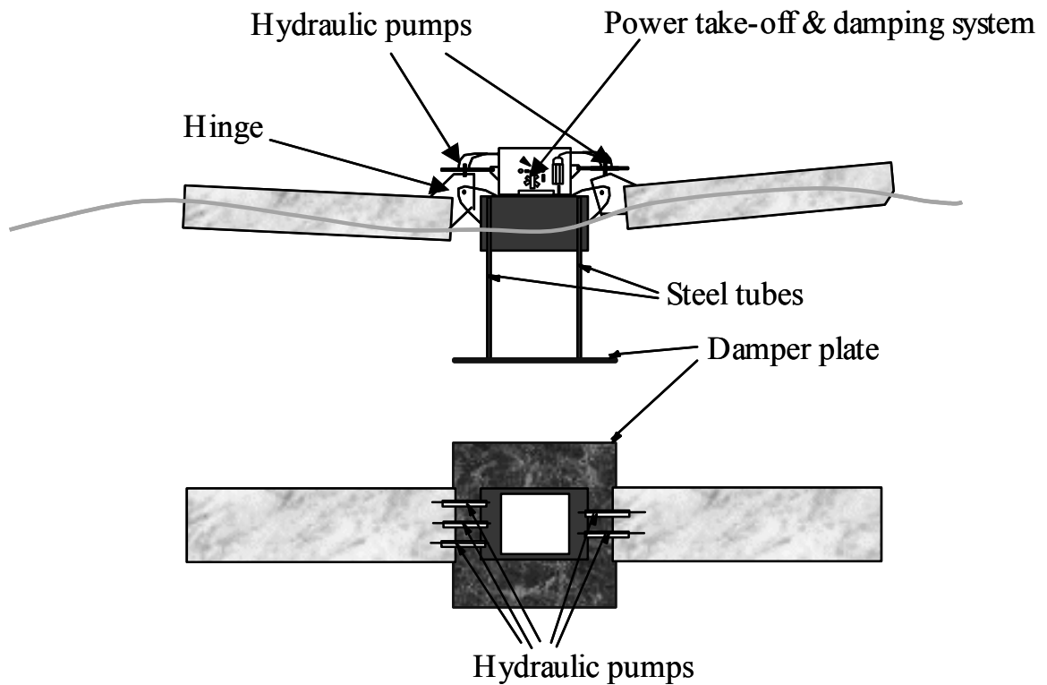
Fig 10 Outline of the McCabe Wave Pump
