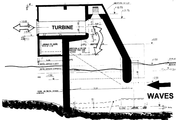
Illustration supplied by IST, Portugal. Fig 4: Outline of the European Pilot Plant
