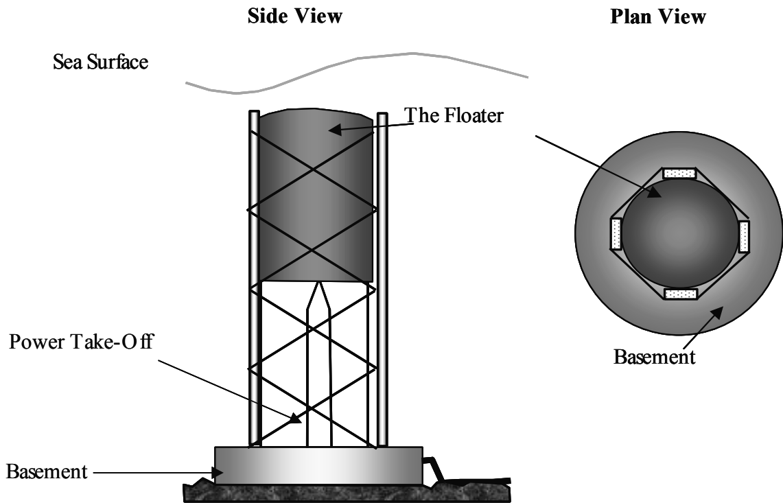
Fig 11 Outline of the Archimedes Wave Swing
