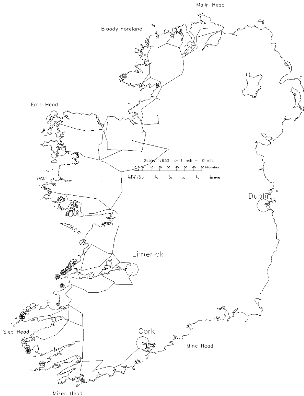
Fig 4. Approximate location of the 38 kV circuits near the west coast
