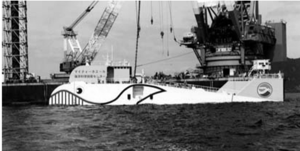
Fig 9 The Mighty Whale Being Launched
